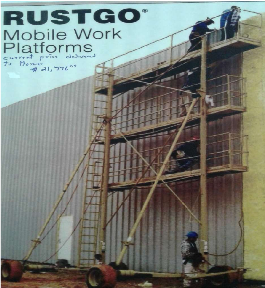
35. Rustgo work platform 32' working height 3 work platforms. Breaks down and assembles with 2 men, and adapts to unlevel ground
